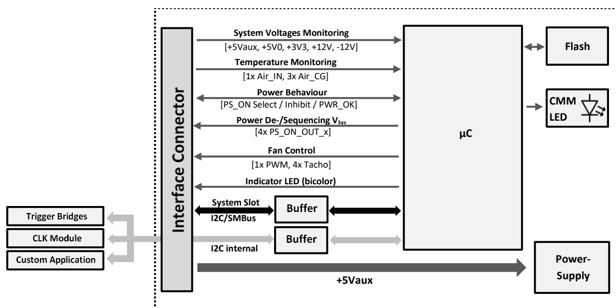
Figure 8: Chassis Management Module (CMM)
