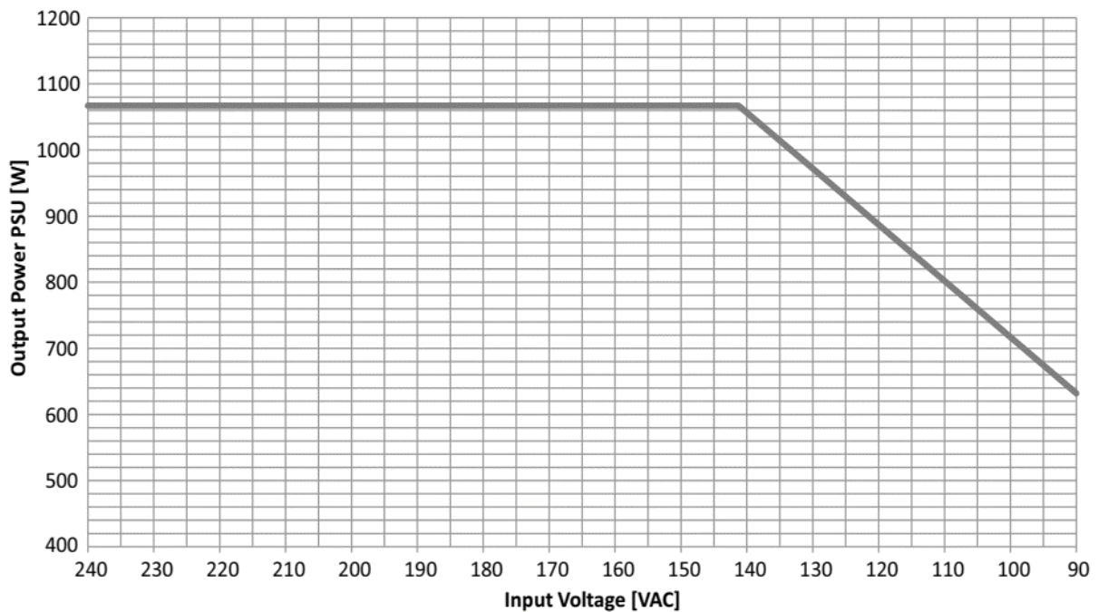
Figure 10: Output Power Derating
