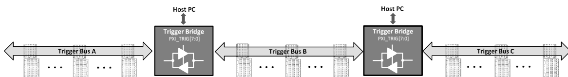
Figure 7: Trigger Bus Segments
