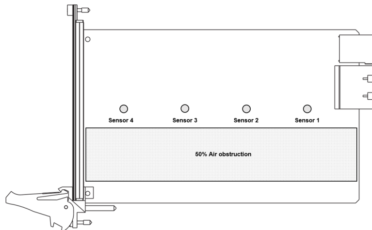
Figure 12: Dummy Impedance Board
