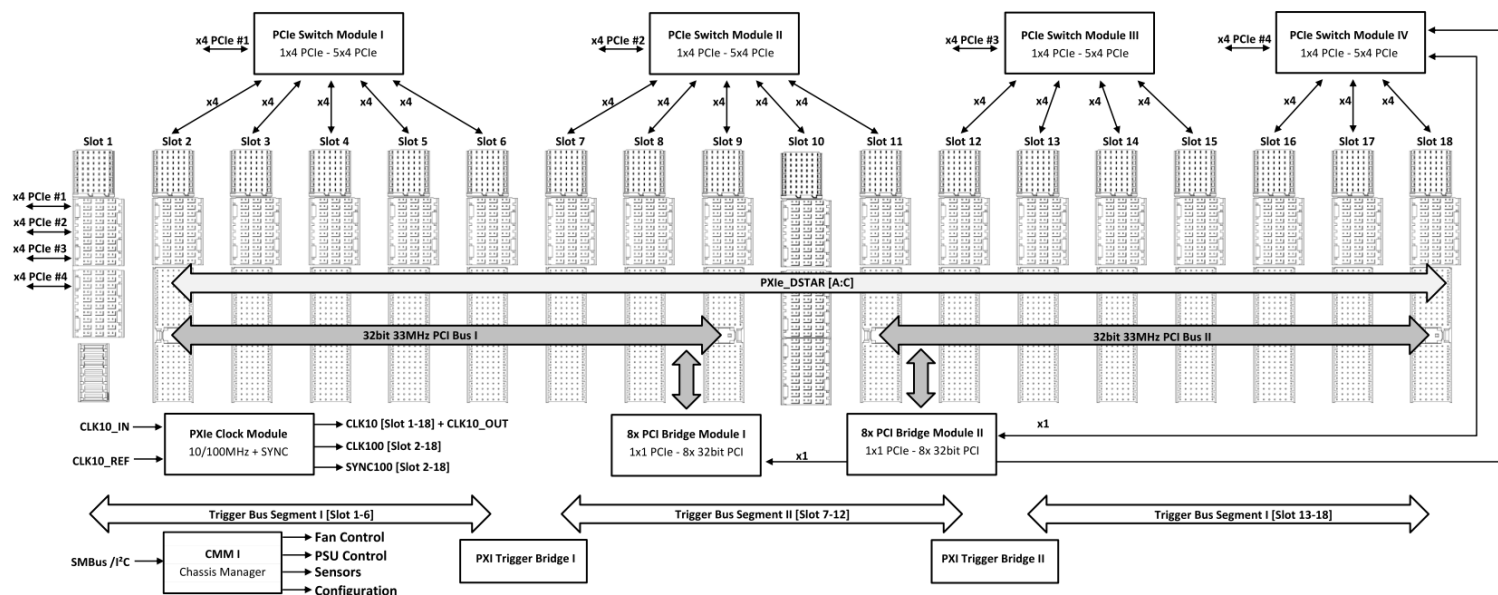
Figure 3: Backplane Topology
