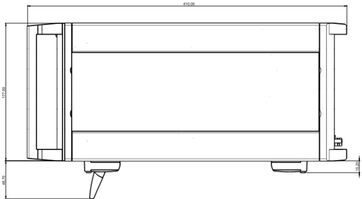
Figure 17: Dimensions Side View
