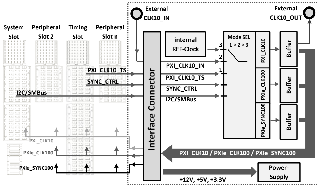
Figure 6: Clock Module
