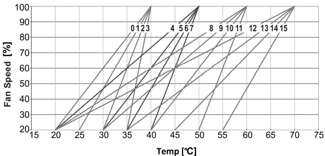
Figure 15: Fan Curves
