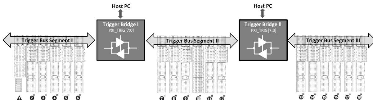
Figure 19: Trigger Bus Segments
