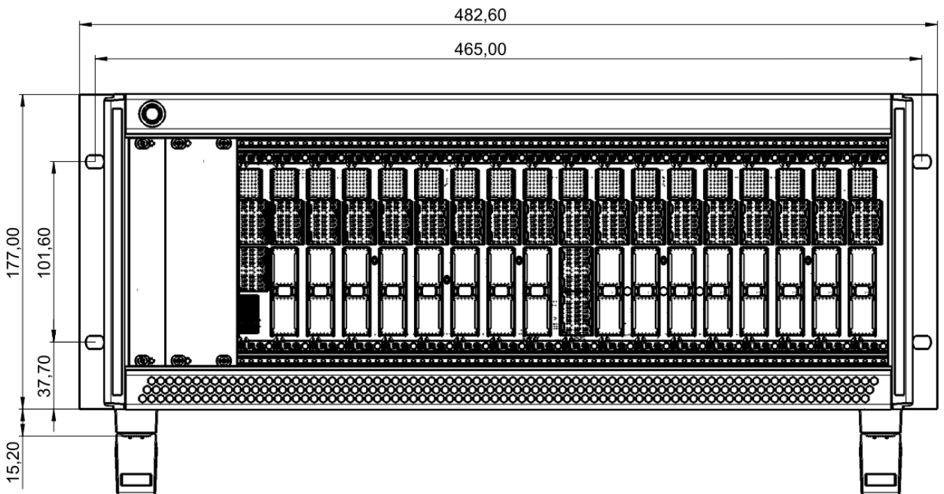
Figure 16: Dimensions Front View
