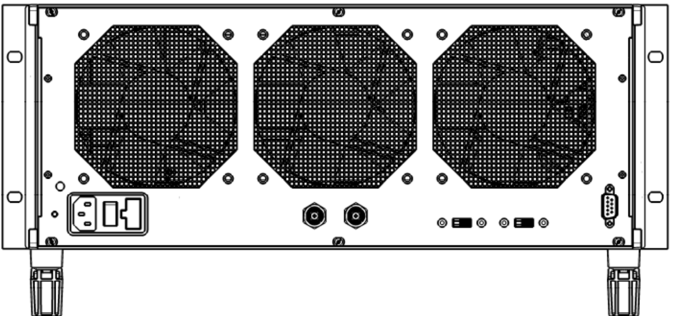
Figure 18: Dimensions Rear View
